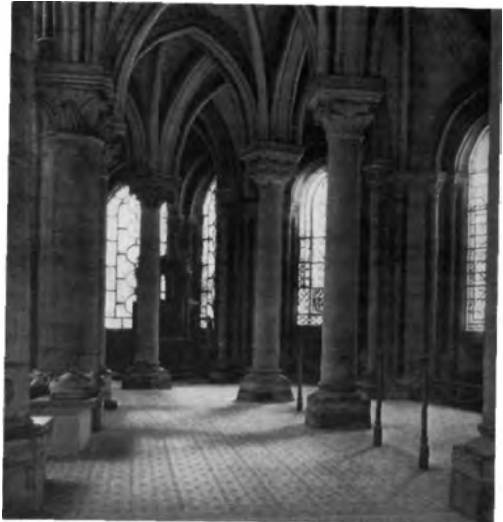
St Denis ambulatory, built between 1111 and 1144) Abbot Suger of St. Denis (1081-1151) was responsible for this building plan for the abbey church of St. Denis. He was not only the regent of France between 1147 and 1149, but also made a name for himself as a writer of the ambulatory shown here, when he saw two features of design typical of Gothic architecture, firstly, the aim was to reduce the masonry to make room for big windows; and secondly, a large number of columns were erected to increase the tectonic stability
