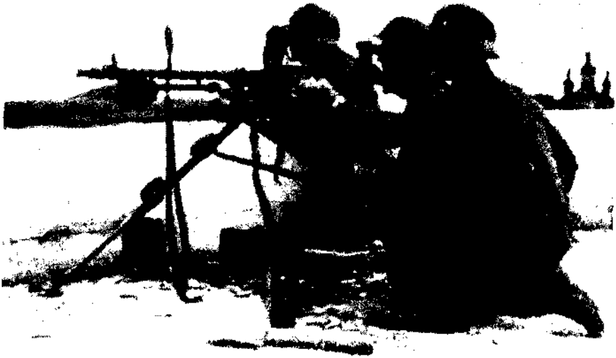
Figure 37.—M.G. 34 in action on tripod mount, with anti-aircraft and telescopic sights.
