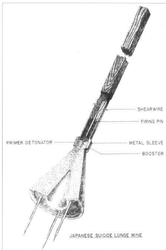
The 2.9kg (6.4lb) of explosives in the warhead of the lunge mine ( shitotsu bakurai ) was pushed back with its detonator onto a firing pin when slammed into the side of a tank. Three 5.25in rods protruding from the base of the cone ensured optimum 'stand-off' for the hollow charge. US troops called this suicide weapon an 'idiot stick', but it did knock out tanks. Circular Type 93 (1933) AT mines ('tape measure mines') were also fastened to the ends of poles for the same purpose.
