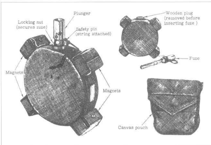
The Japanese Type 99 (1939) AT charge (99 hako-bakurai ) was small (about 4¾ in x 1½ in without the four magnets), but if two or more could be fastened together they caused a great deal of concern to tankers (see Plate H). It was issued in a canvas carrying pouch, with the fuze packed in a two-piece metal tube under the pouch flap.
