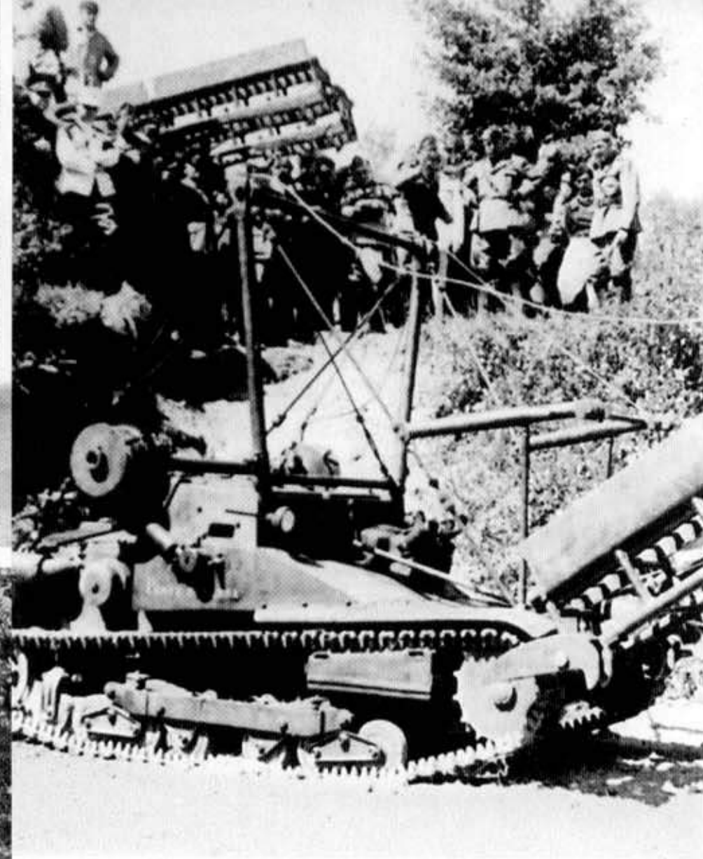
(Left) Army officers demonstrate the CV 33 Passerella (Footbridge) bridgelayer to the Duce (Leader), Benito Mussolini (hands on both hips), during maneuvers in the Summer of 1936. This was the third most important CV 33 variant, after the standard machine gun and flame thrower variants. Mussolini served as a soldier on the Isonzo Front facing Austria-Hungary during World War One.
